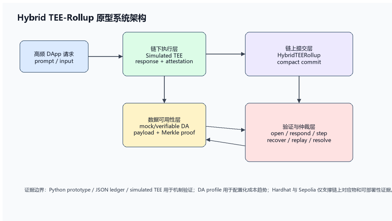
图 1 Hybrid TEE-Rollup 原型系统架构 Fig.1 Prototype architecture of Hybrid TEE-Rollup
