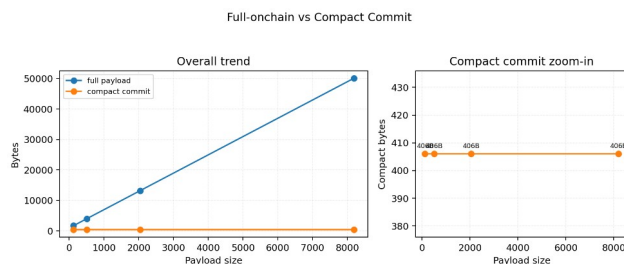
图 3 完整负载与紧凑提交的字节规模对比 Fig.3 Byte-size comparison between full payloads and compact commits
