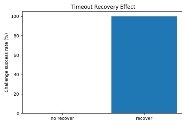
图 6 超时恢复对挑战完成率的影响 Fig.6 Impact of timeout recovery on challenge completion rate
