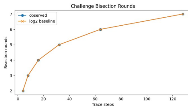
图 5 二分挑战轮次与轨迹步数的关系 Fig.5 Relationship between bisection rounds and trace steps
