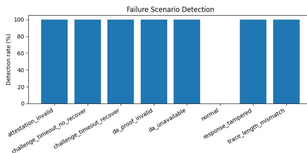
图 7 失败场景检测与仲裁结果 Fig.7 Detection and arbitration outcomes under failure scenarios
